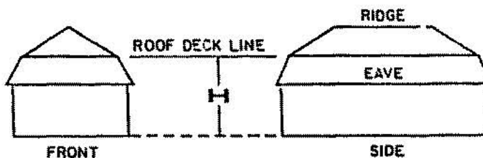
MANSARD ROOF
