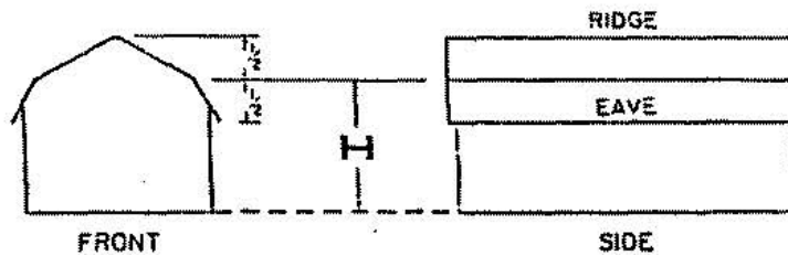
GAMBREL ROOF
